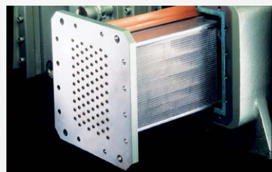
Water-in-tube intercooler and aftercooler bundles slide out for easy inspection and cleaning.
